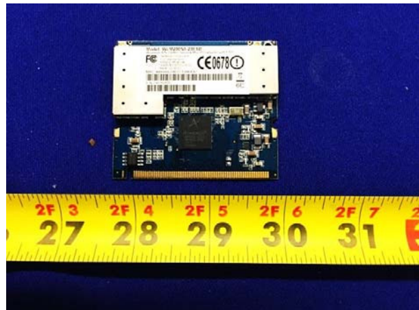
EUT Radio with Shielding Top View
