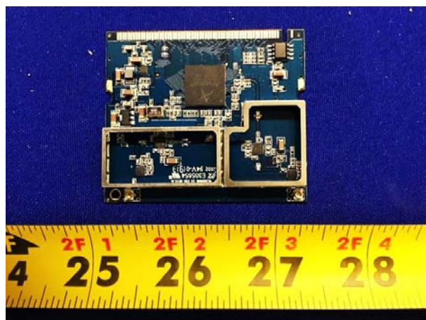
EUT Radio without Shielding Top View
