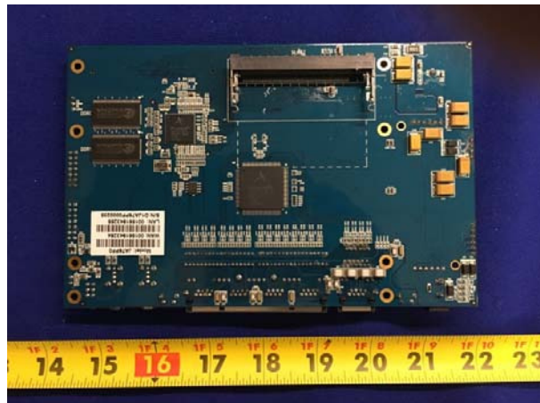
PCBA Bottom View
