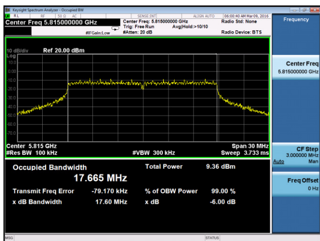
99% & 6dB BW – 20M 5815MHz
