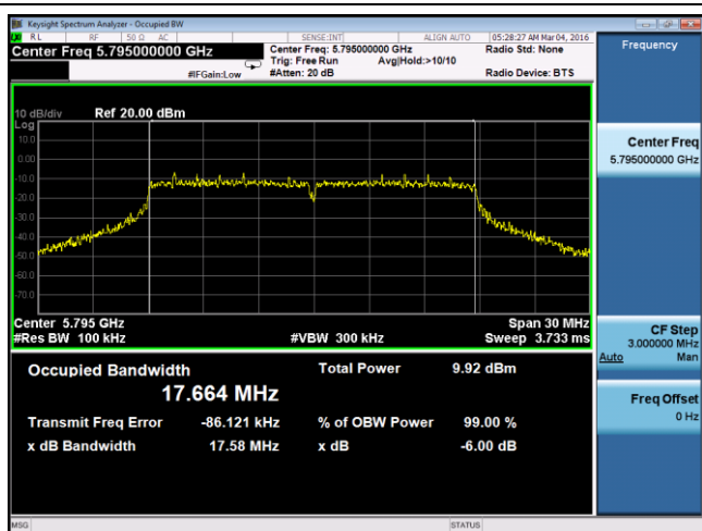
99% & 6dB BW – 20M 5795MHz
