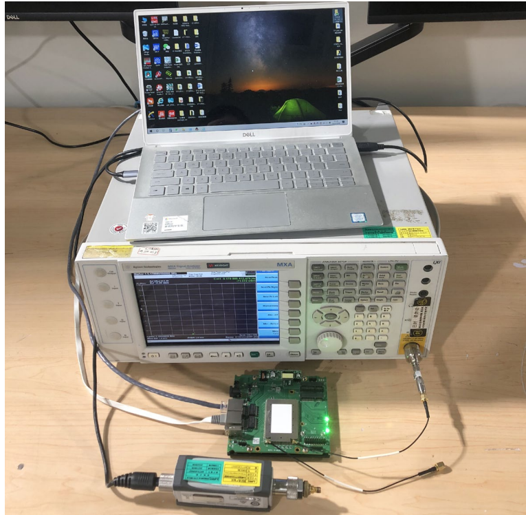
Description: DFS Test Setup
