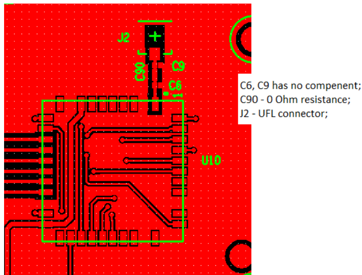
Antenna matching peripheral circuit PCB layout
