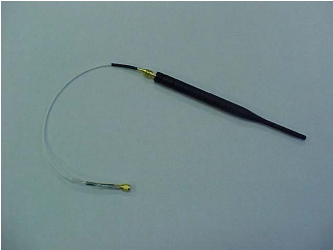
Photo Six – External Alternate Antenna with Coax Cable
