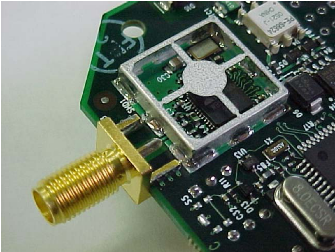
Photo Five – Internal PCB RF Section with Antenna Connection
