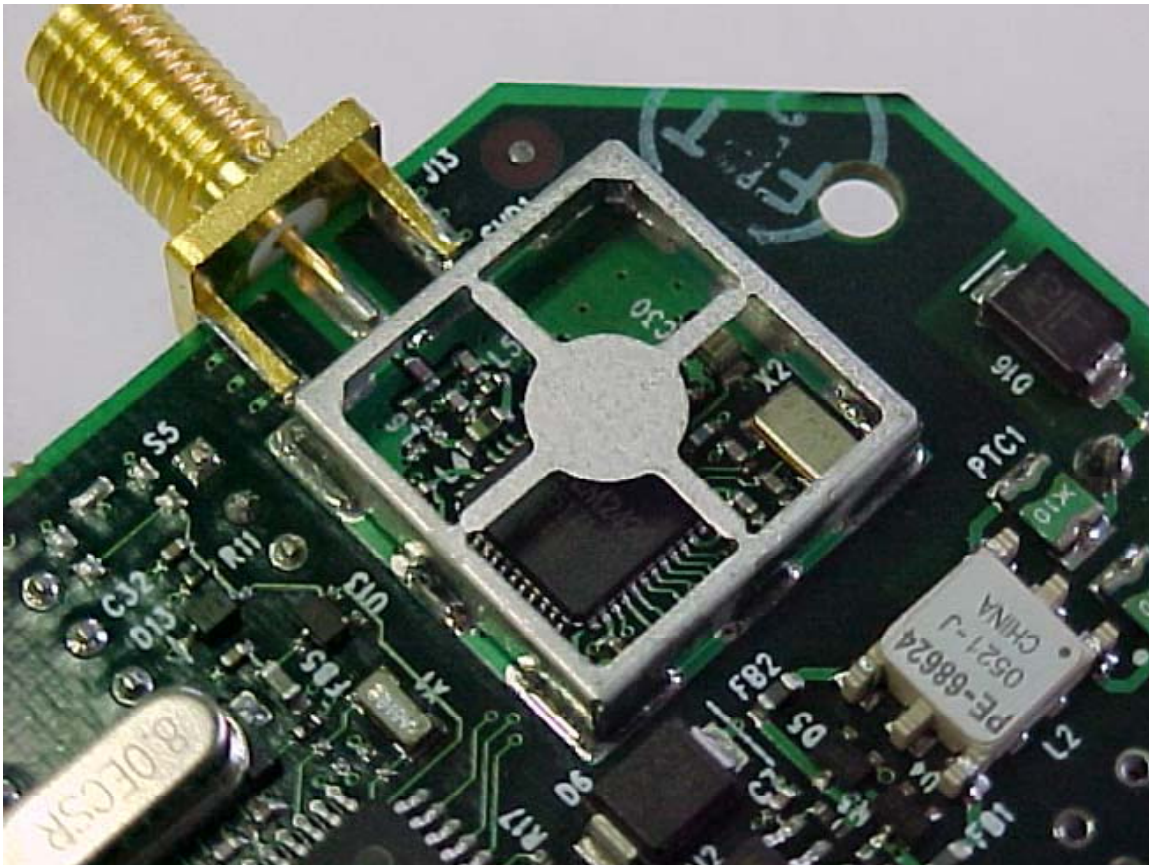
Photo Four – Internal PCB RF Section Close-up
