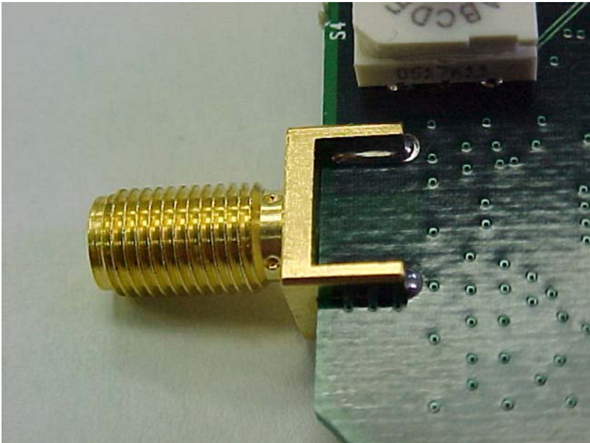
Photo Six – Internal PCB RF Antenna Connection
