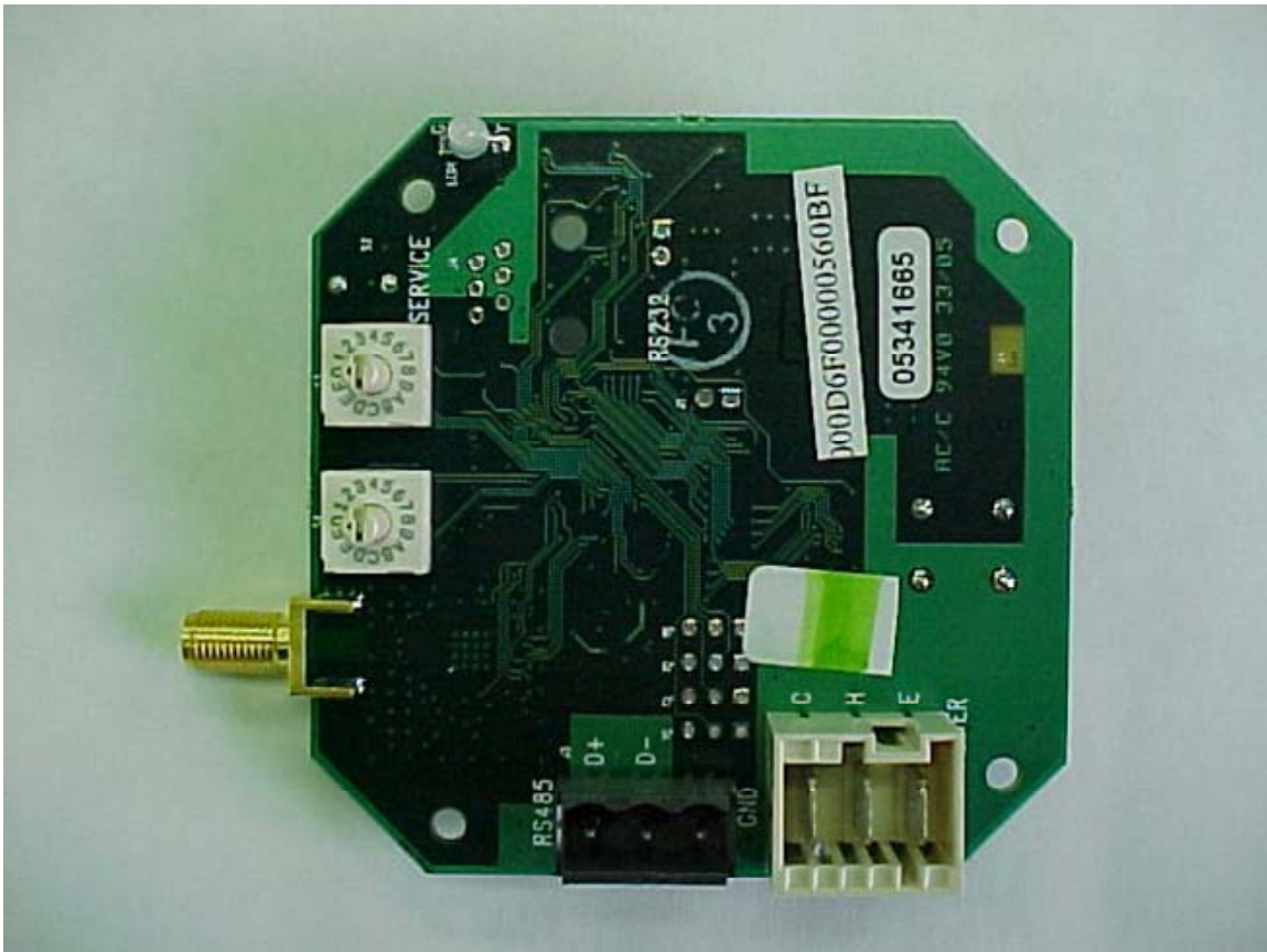
Photo Two – Internal PCB Connector Side
