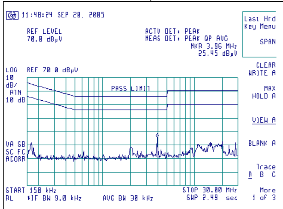
Channel 0, Line 1
