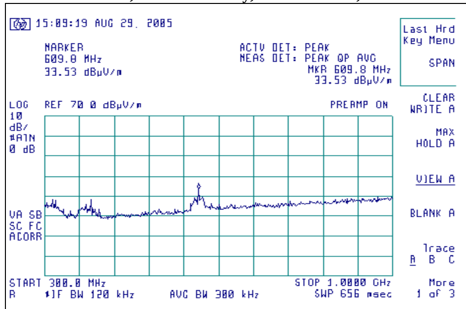
Channel F, Vertical Polarity, 300-1000 MHz, unit flat
