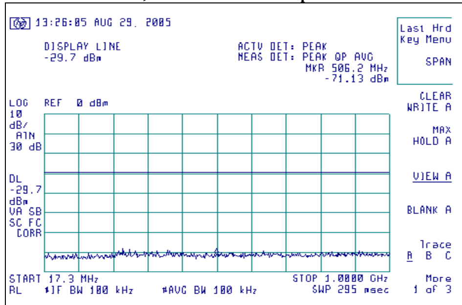
Channel 0, shown from 17 MHz up to 1000 MHz
