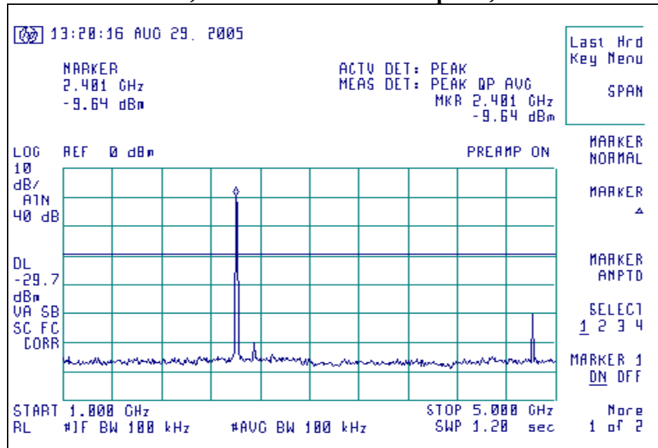
Channel 0, shown from 1000 MHz up to 5,000 MHz
