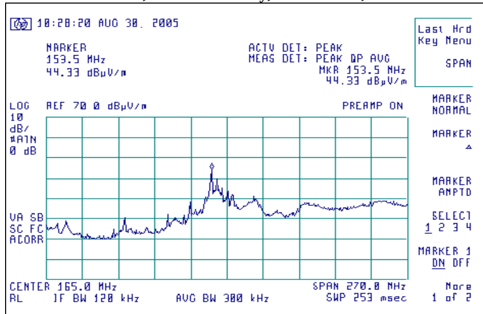
Channel F, Vertical Polarity, 30-300 MHz, unit flat
