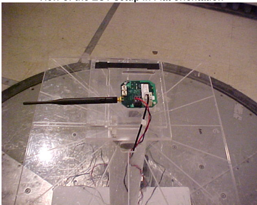
View of the EUT setup in Flat orientation
