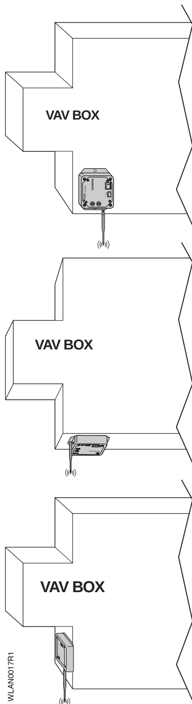
Figure 2. FLNX Mounting Options, no enclosure.
