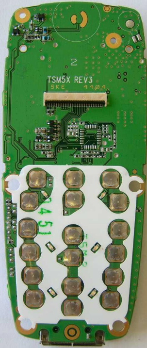
TSM2 PCB front view
