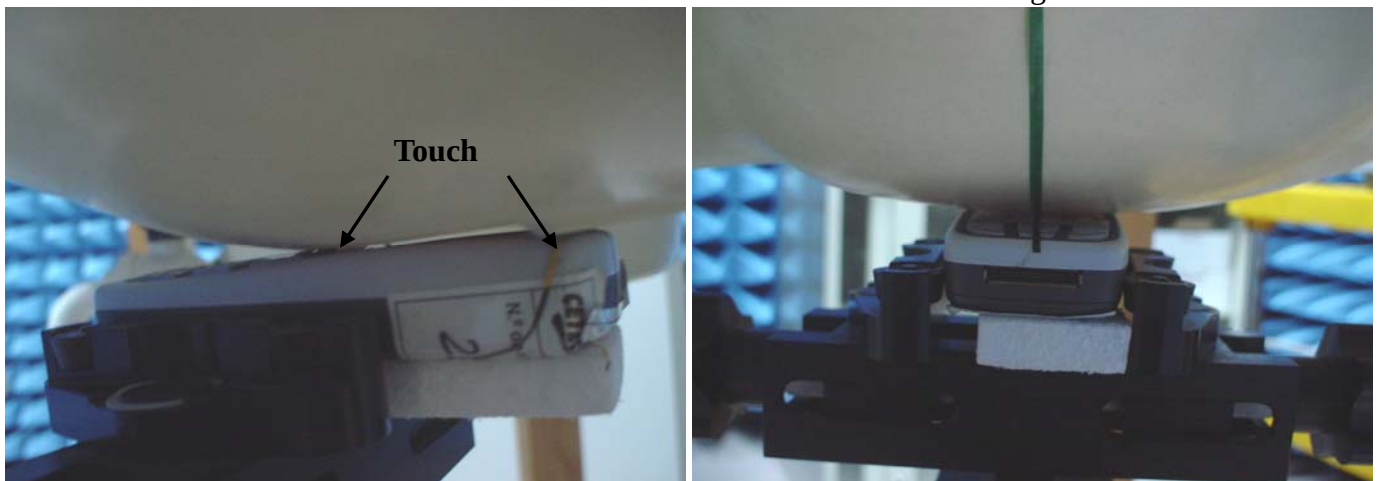
Fig.5 Left Head Section / Cheek-Touch Position
