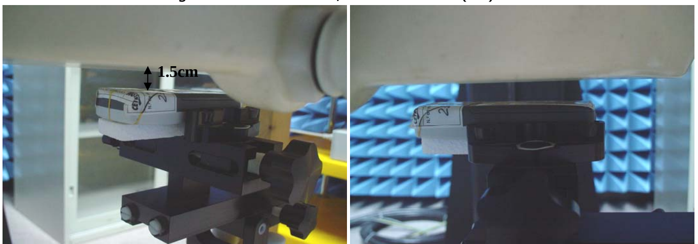
Fig.6 Left Head Section / Ear-Tilt Position(15°)
