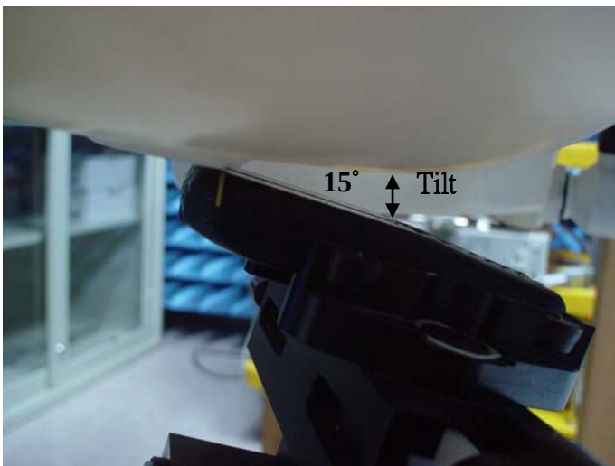
Fig.4 Right Head Section / Ear-Tilt Position(15°)
