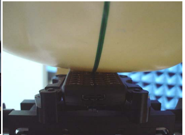
Fig.3 Right Head Section / Cheek-Touch Position
