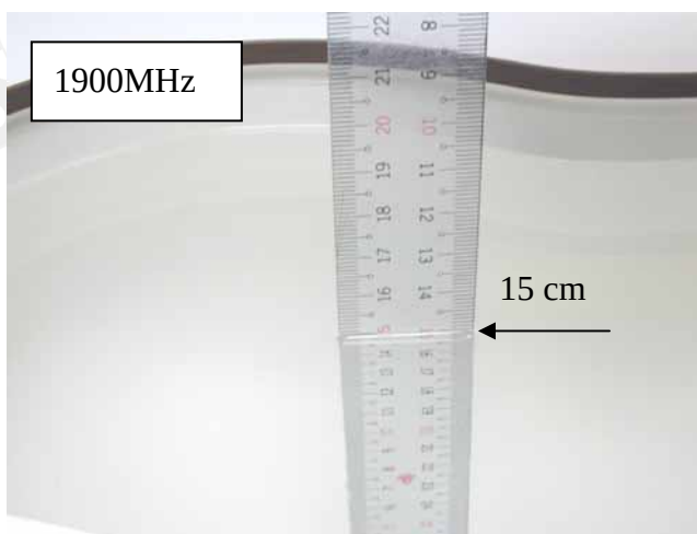
Fig.2.2 Photograph of the Tissue Simulant Fluid liquid depth 15cm for Right-head Side
