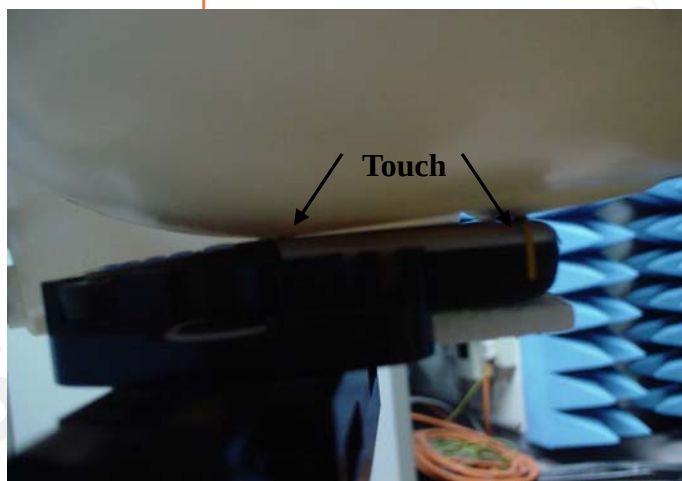
Fig.5 Left Head Section / Cheek-Touch Position
