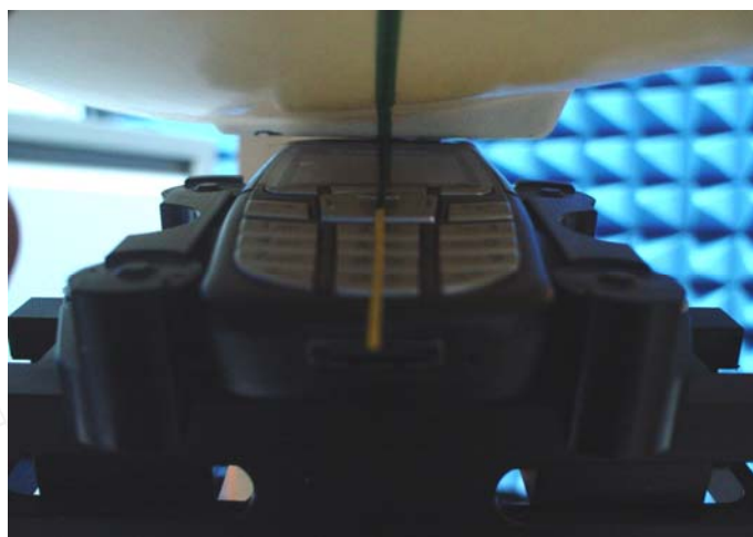
Fig.4 Right Head Section / Ear-Tilt Position(15°)
