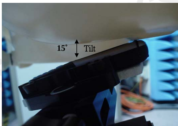
Fig.6 Left Head Section / Ear-Tilt Position(15°)
