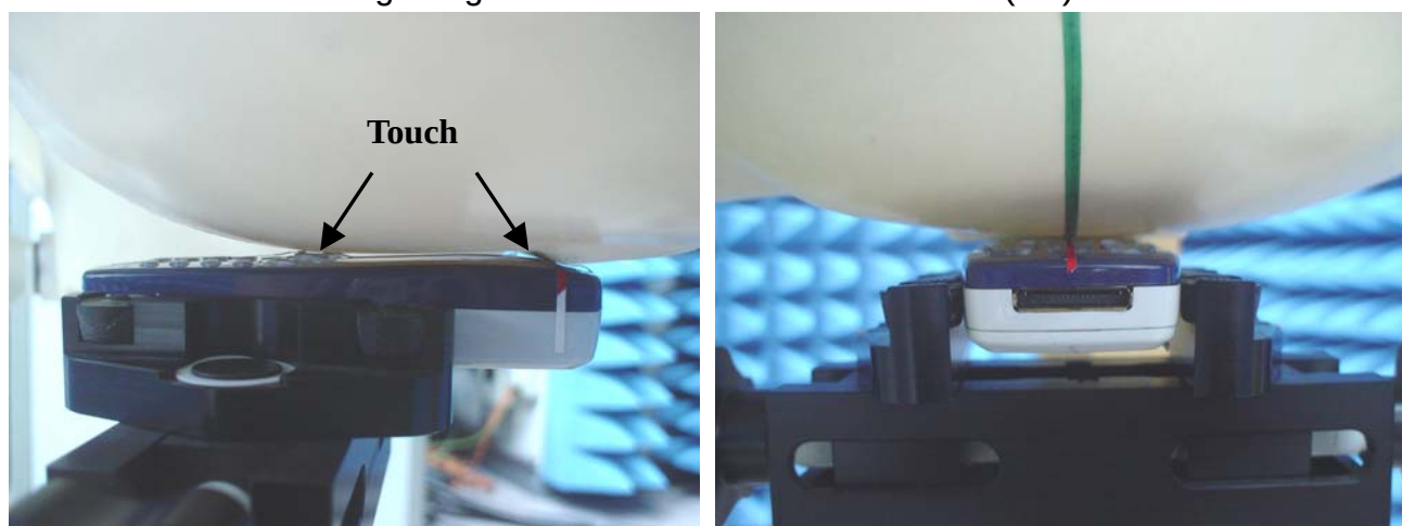
Fig.5 Right Head Section / Ear-Tilt Position(15°)
