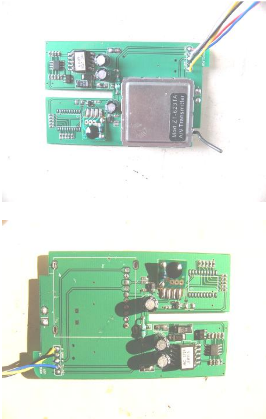
Main & RF board component side
