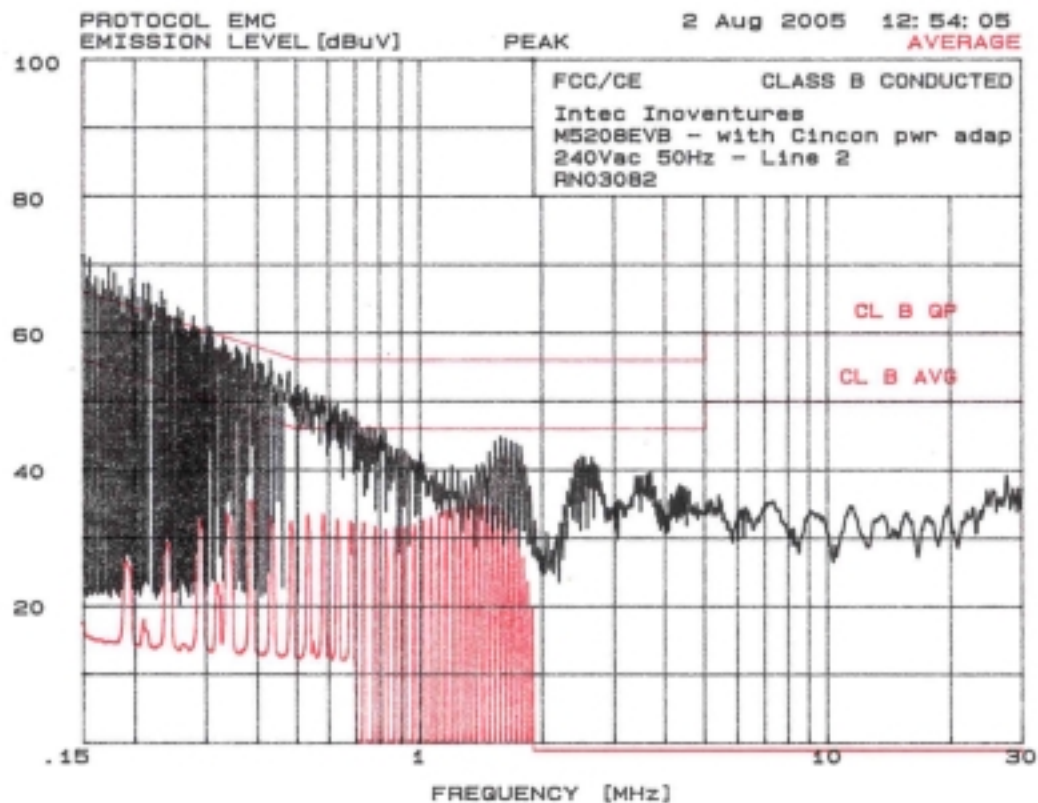
Conducted Emissions 240Vac 50 Hz Line 2
