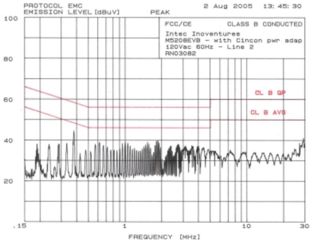
Conducted Emissions 120Vac 60 Hz Line 2
