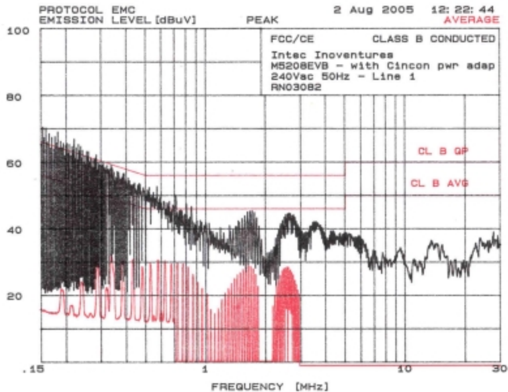
Conducted Emissions 240Vac 50 Hz Line 1
