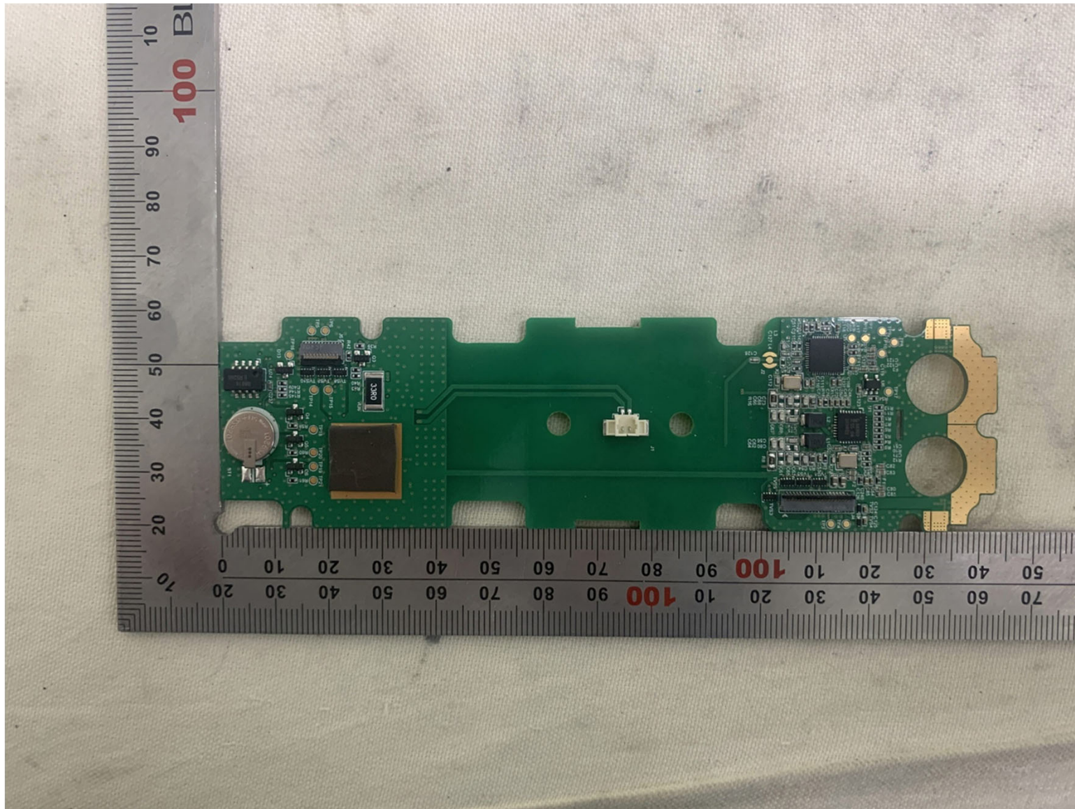
RF BOARD Rear
