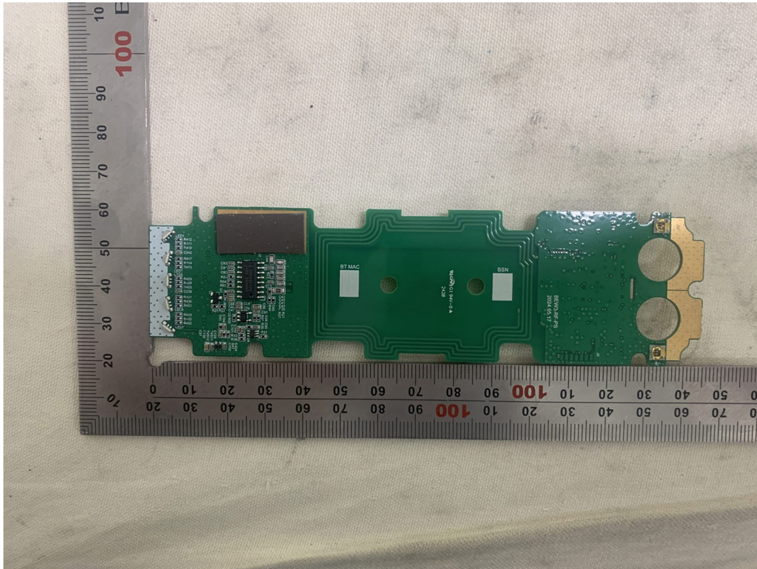
RF BOARD Front
