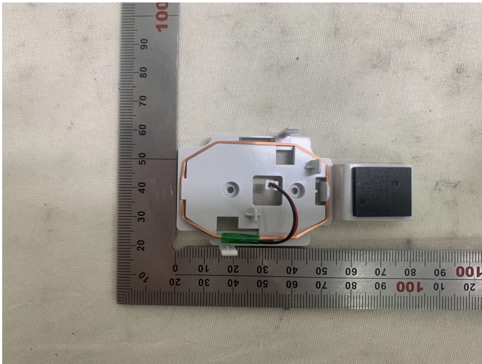
COIL ANTENNA
