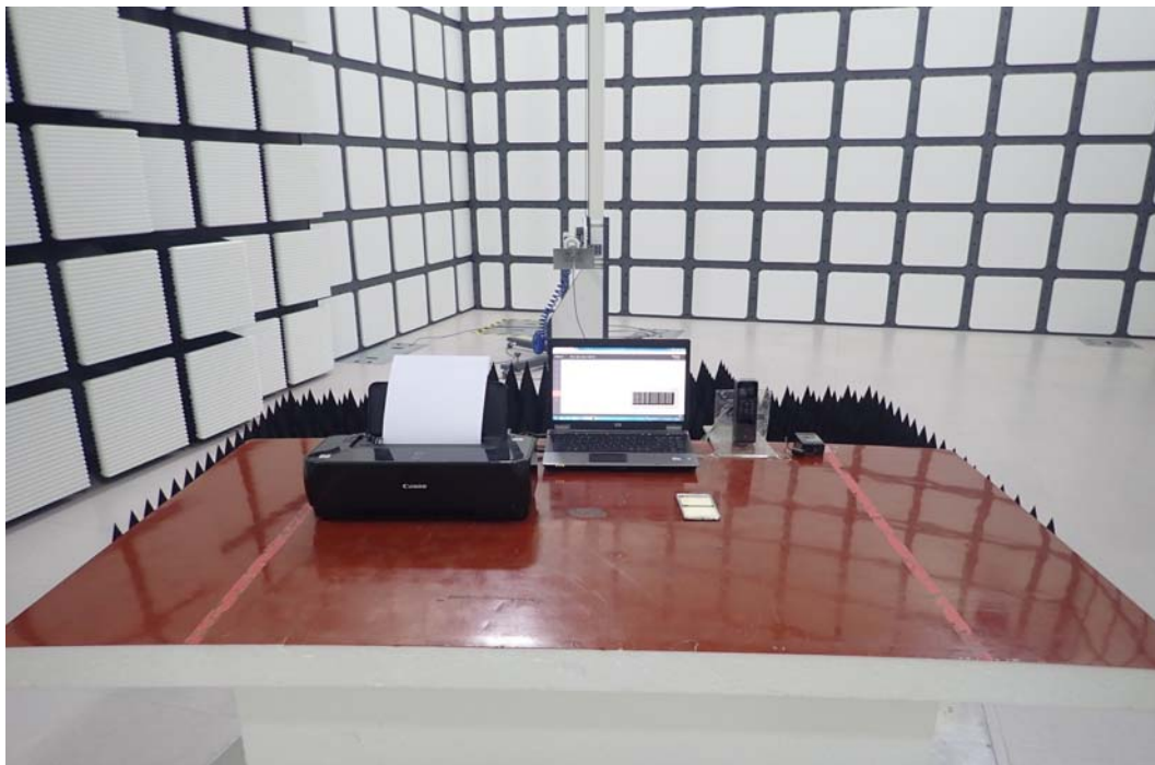
Above 1 GHz 2.2.1 Front
