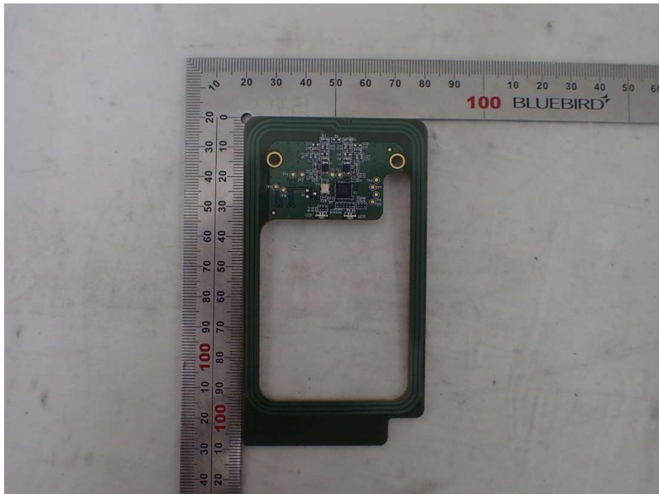
< Antenna Board – Front >
