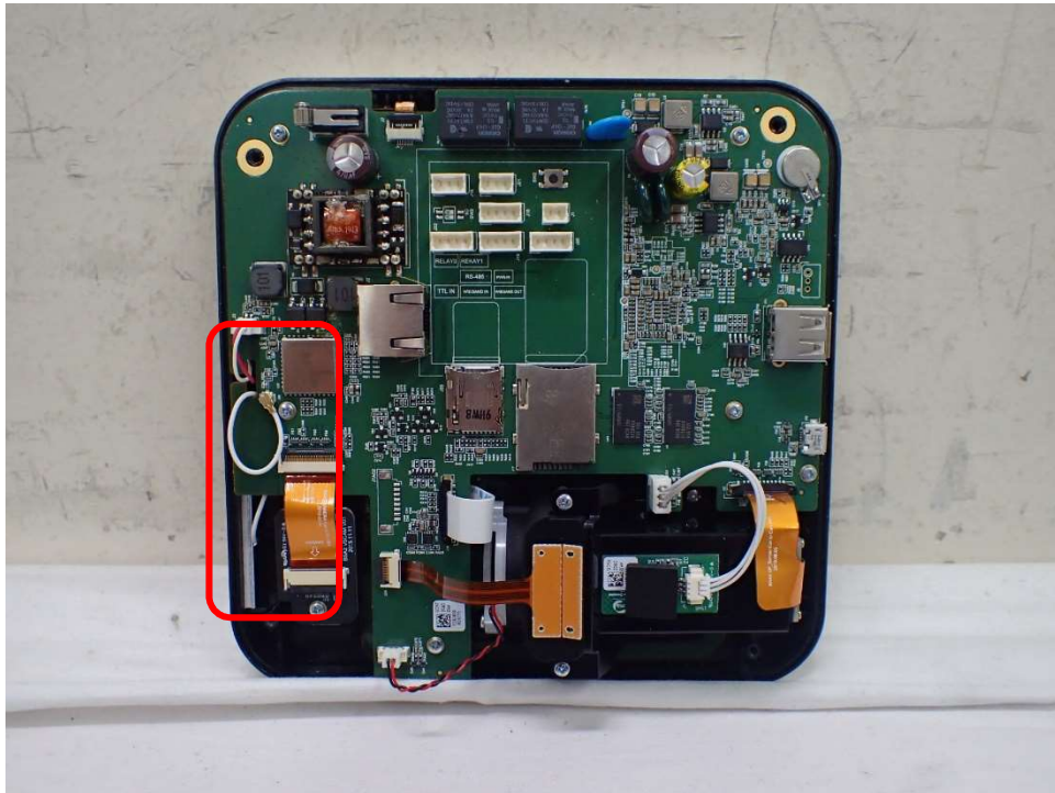
<Inside Photo – 2.4GHz Antenna port>
