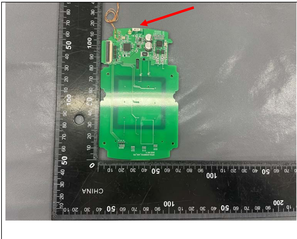
Chip Antenna (Bluetooth LE)
