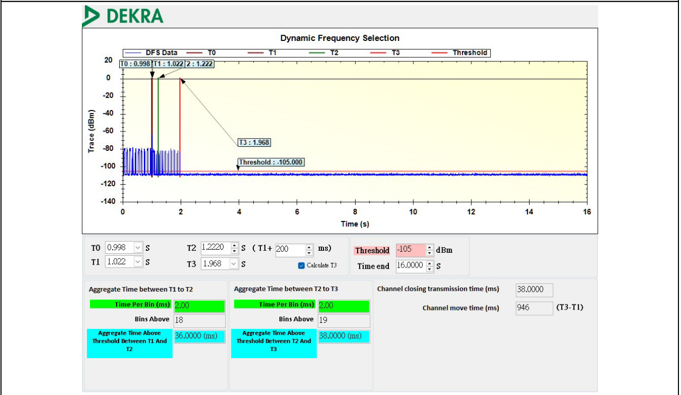
Channel Move Time and Channel Closing Transmission Time - 802.11ax (160 MHz), 5250 MHz
