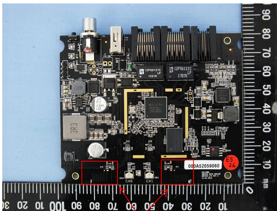
Antenna location
