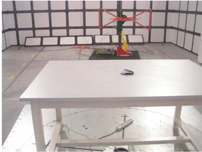
Transmitting Mode: Radiated Emissions-Front View
