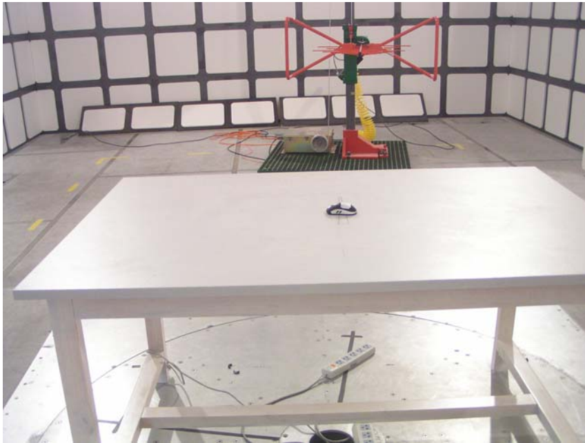
Radiated Emissions-Front View
