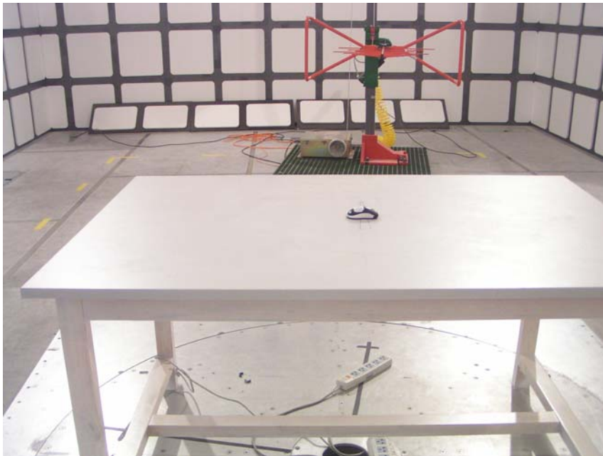
Radiated Emissions-Rear View
