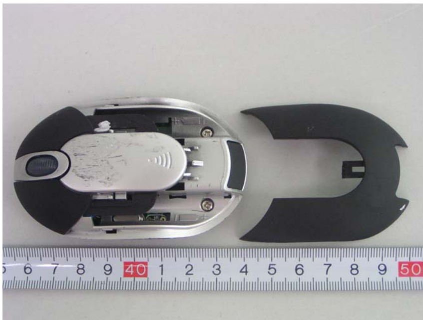
EUT – Uncover View
