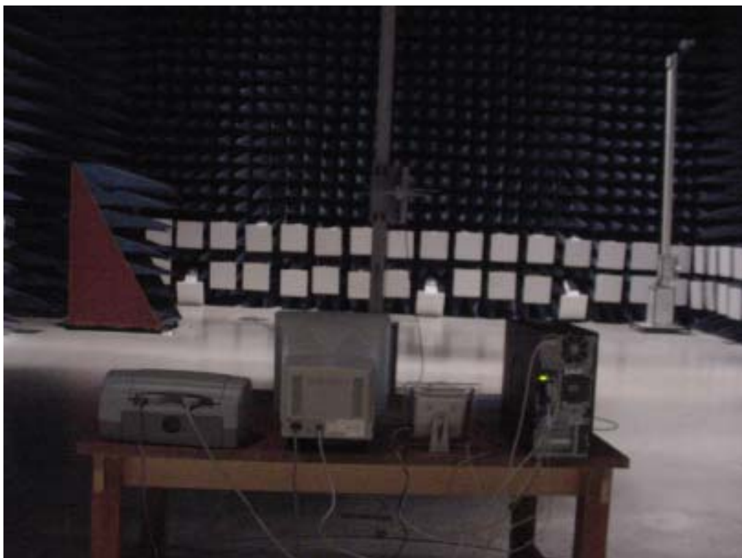
< REAR PHOTOGRAPH OF RADIATED DISTURBANCE >
