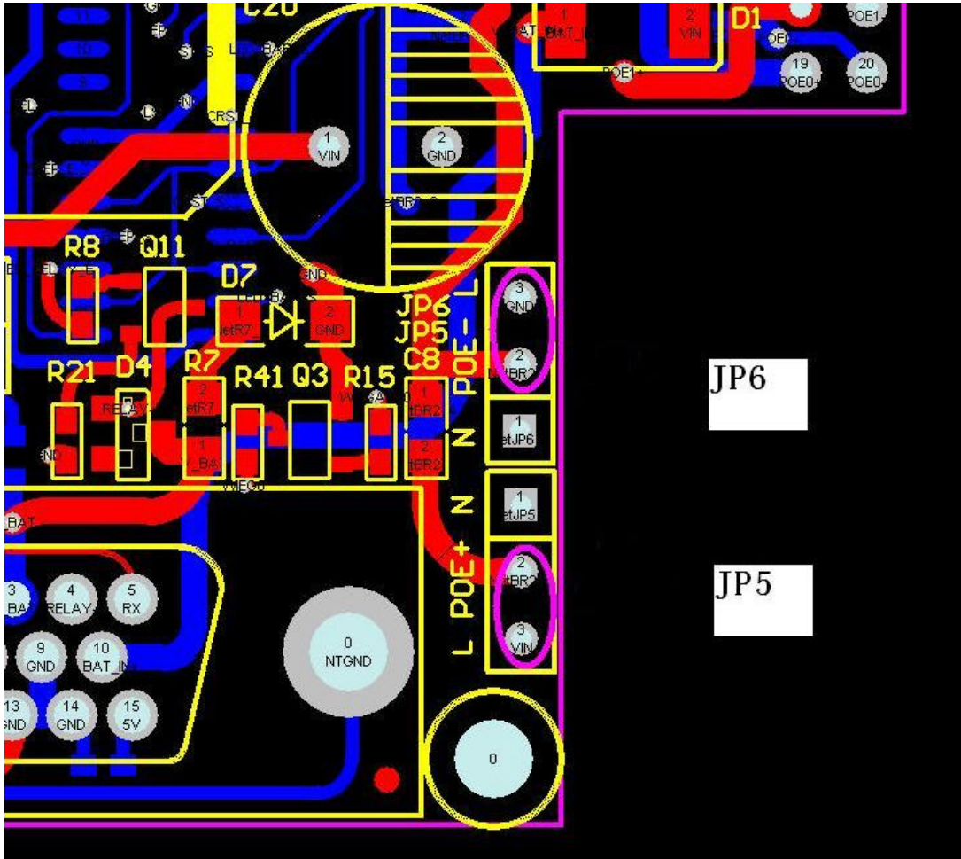
Figure 1.2 Nonstandard POE Device Supply
