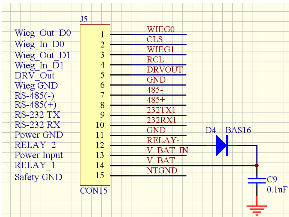
Figure 2.1 DB15 Definition
