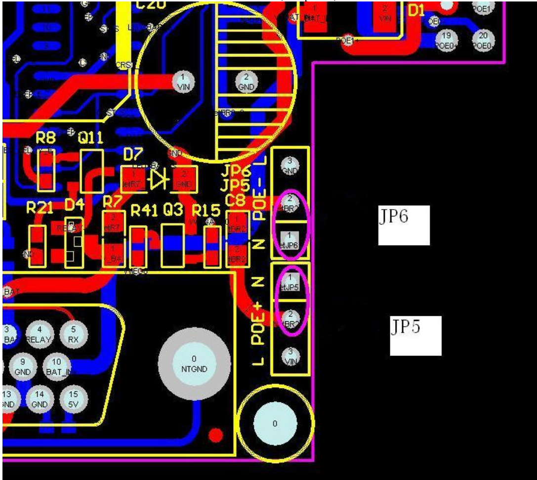
Figure 1.1 Standard POE Device Supply
