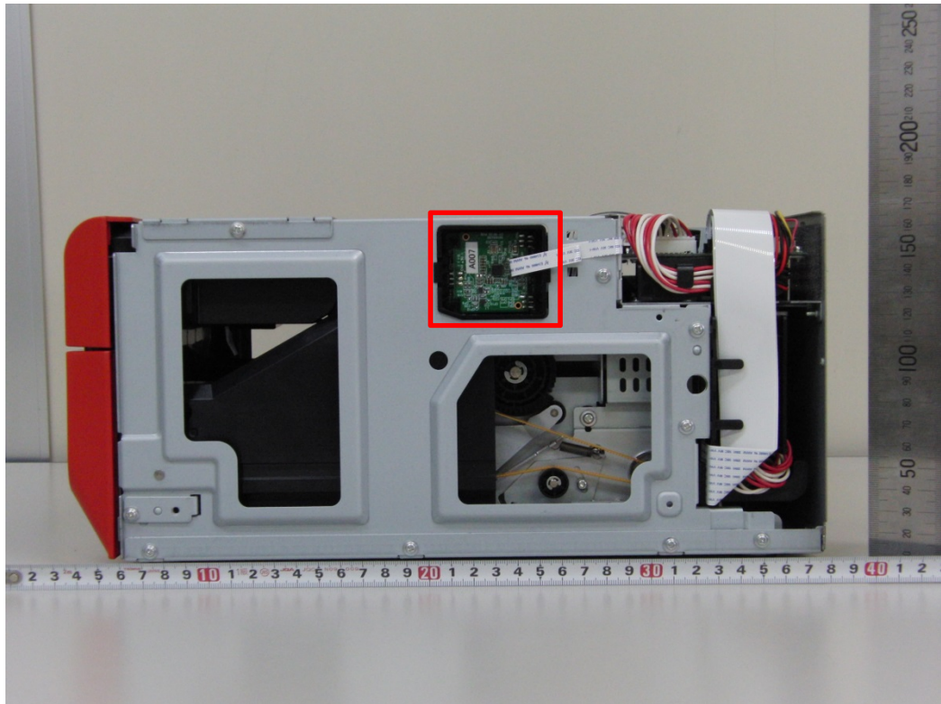
Location of RFID Module
