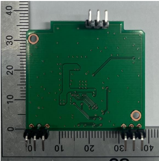
Control PCB
