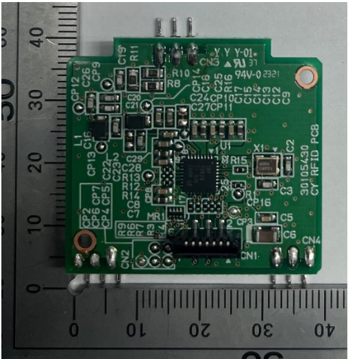
Control PCB
