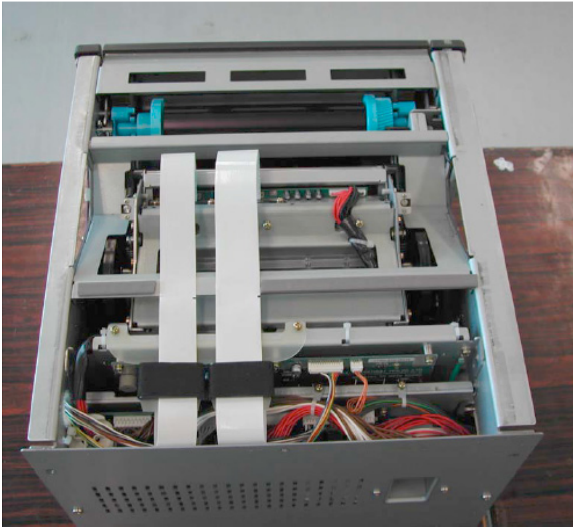
Photograph 9 - Internal Top View of the CV01-H01
