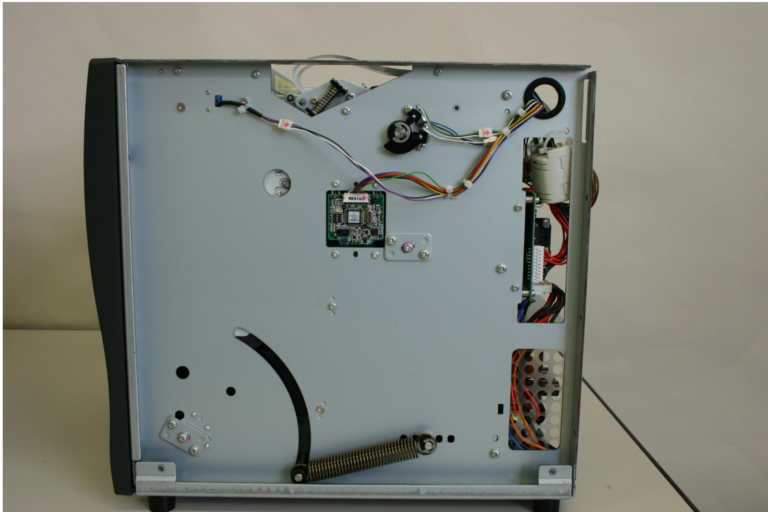
Figure 9.0-9 PHOTO PRINTER CV-01 Internal View- LEFT
