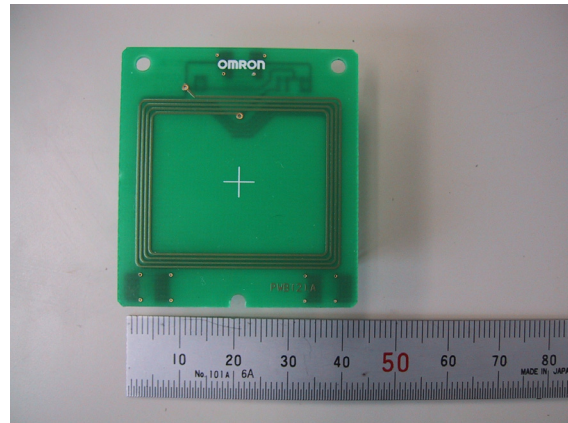
Figure 9.0-11 TOP and BOTTOM VIEW OF RFID Reader/Writer Module ANT BORAD
