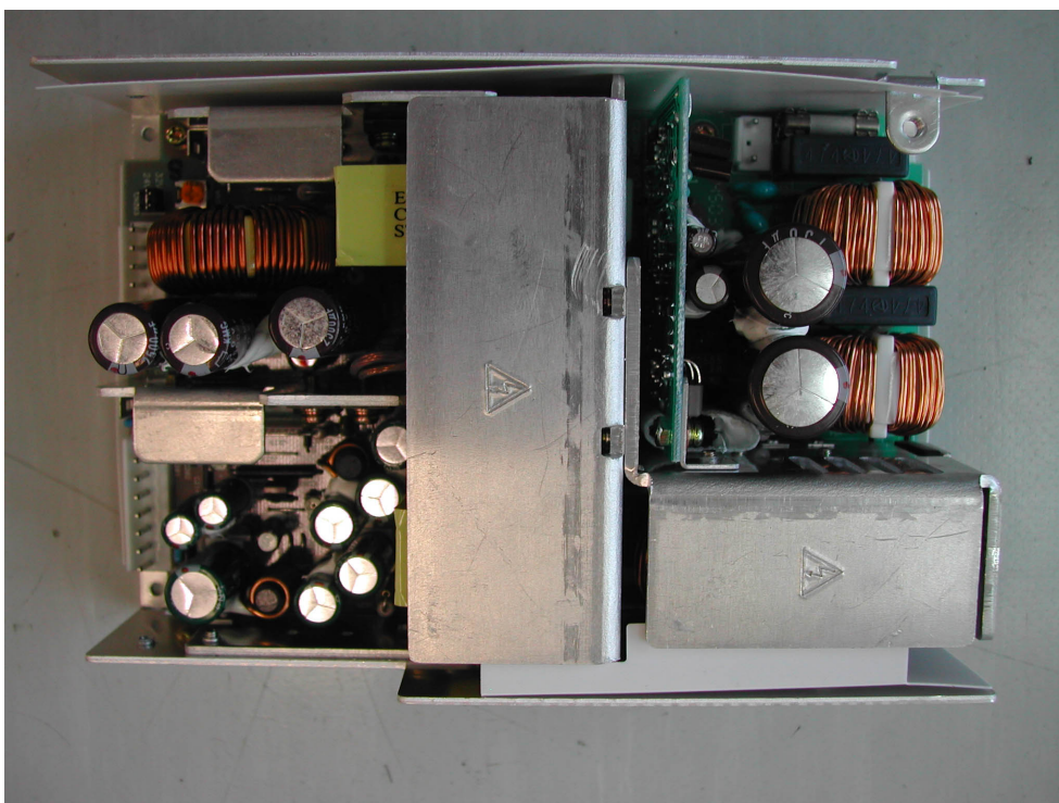
Figure 9.0-2 POWER SUPPLY UNIT
