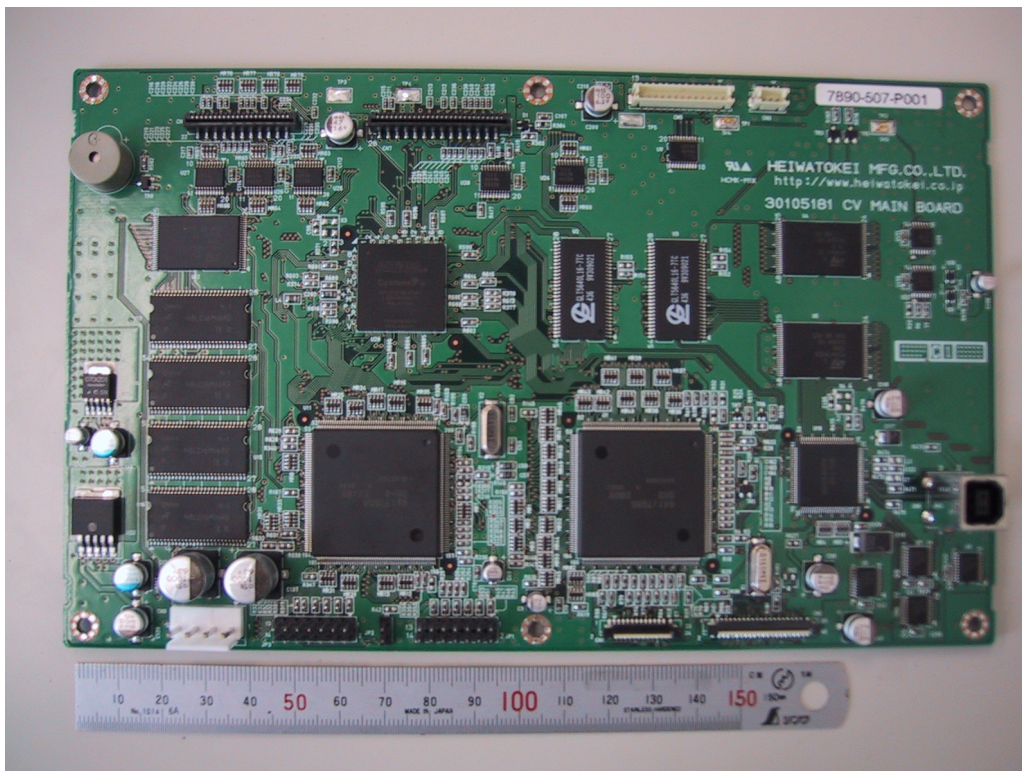
Figure 9.0-5 TOP VIEW OF MAIN BORAD
