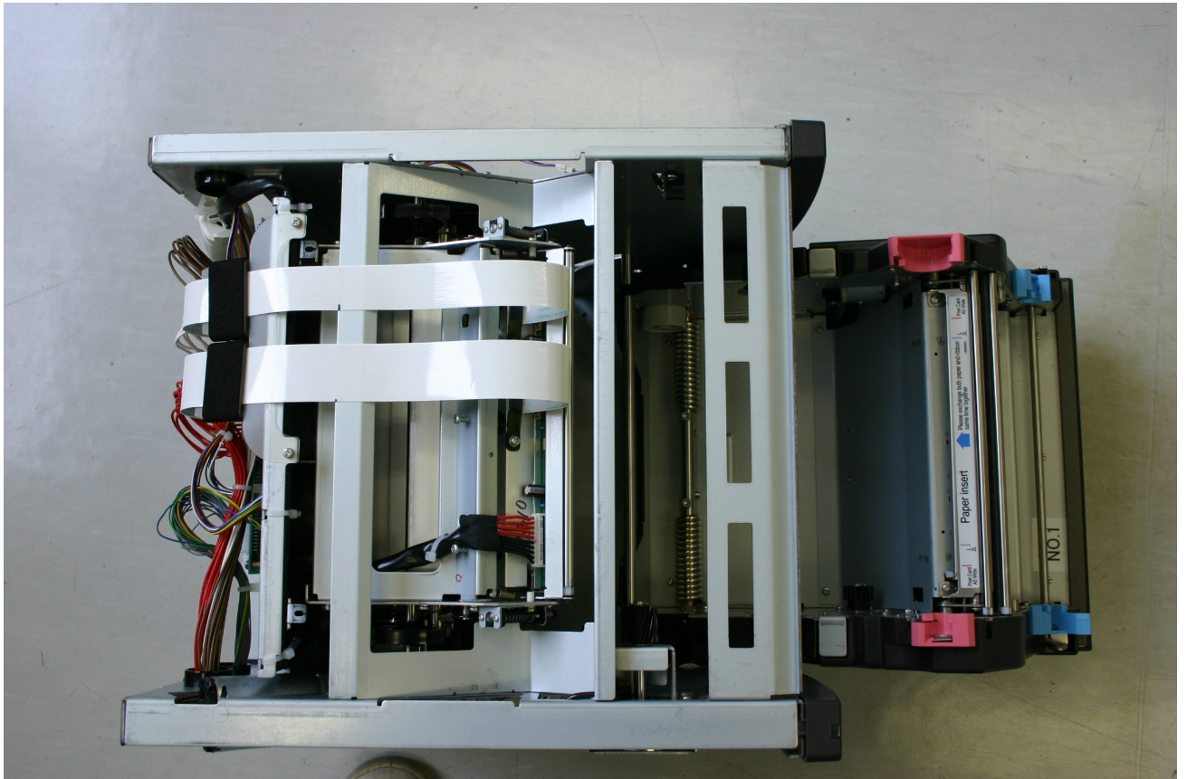
Figure 9.0-12 PHOTO PRINTER CW-01 Internal View- TOP
