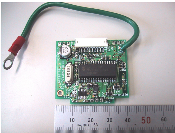
Figure 9.0-9 PHOTO PRINTER CV-01 Internal View- LEFT
