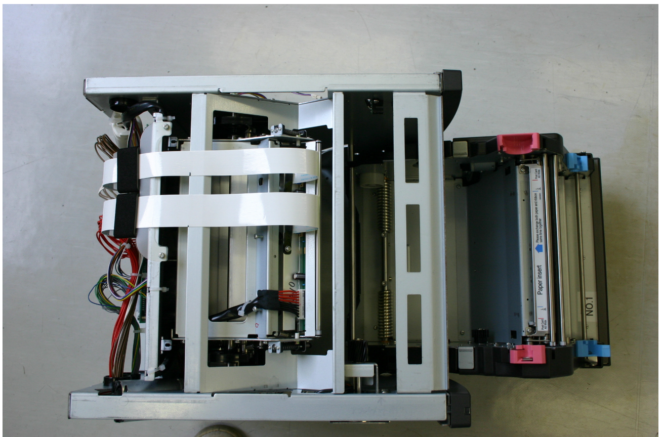
Figure 9.0-12 PHOTO PRINTER CW-01 Internal View- TOP
