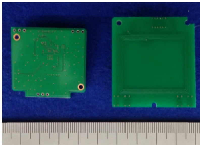
Control PCB
