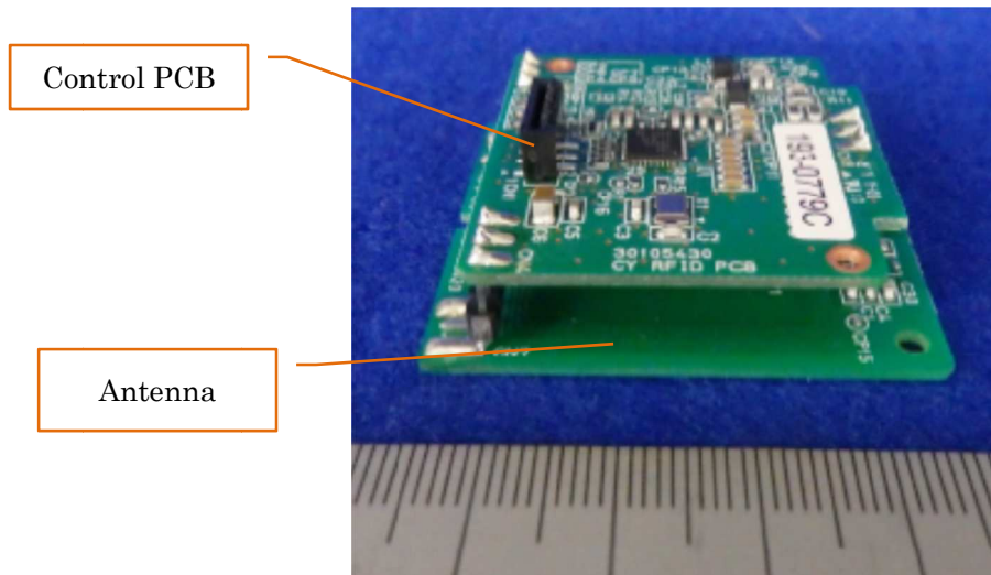
Control PCB
