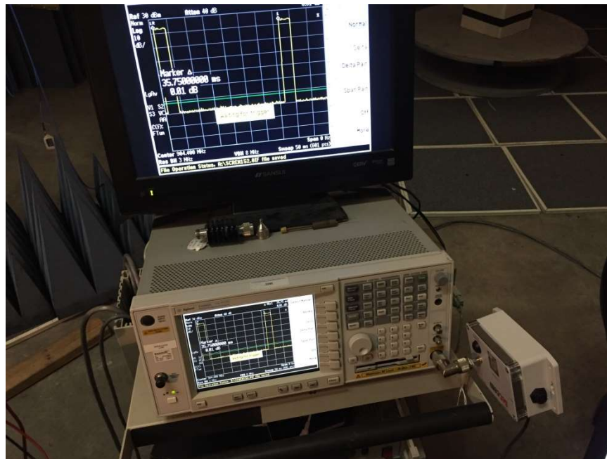
Antenna Port Measurements; Power, PSD, Bandwidth, Duty Cycle
