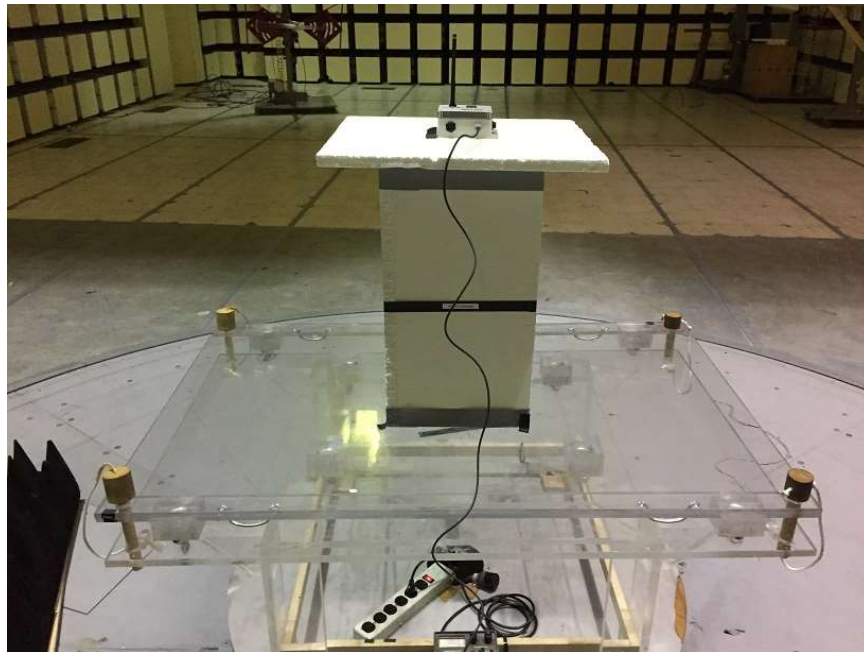
Radiated Emissions > 1 GHz; Transmit and Receive Modes; Back
