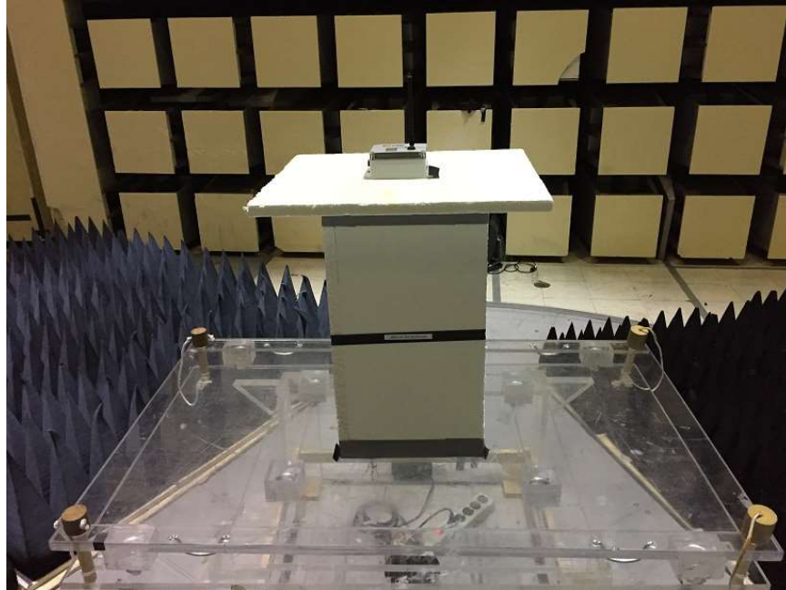
Radiated Emissions > 1 GHz; Transmit and Receive Modes; Front
