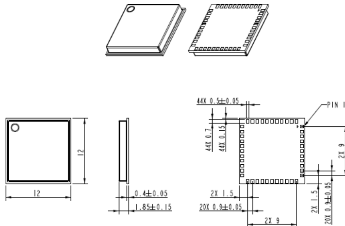
TOLERANCE UNLESS OTHERWISE SPECIFIED: ±0.1mm
