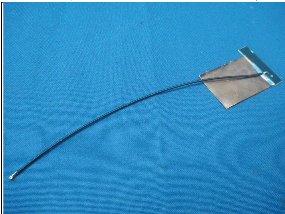
Antenna 2 (Brand: Walsin / Model: RFPCA310715EMLB301)
