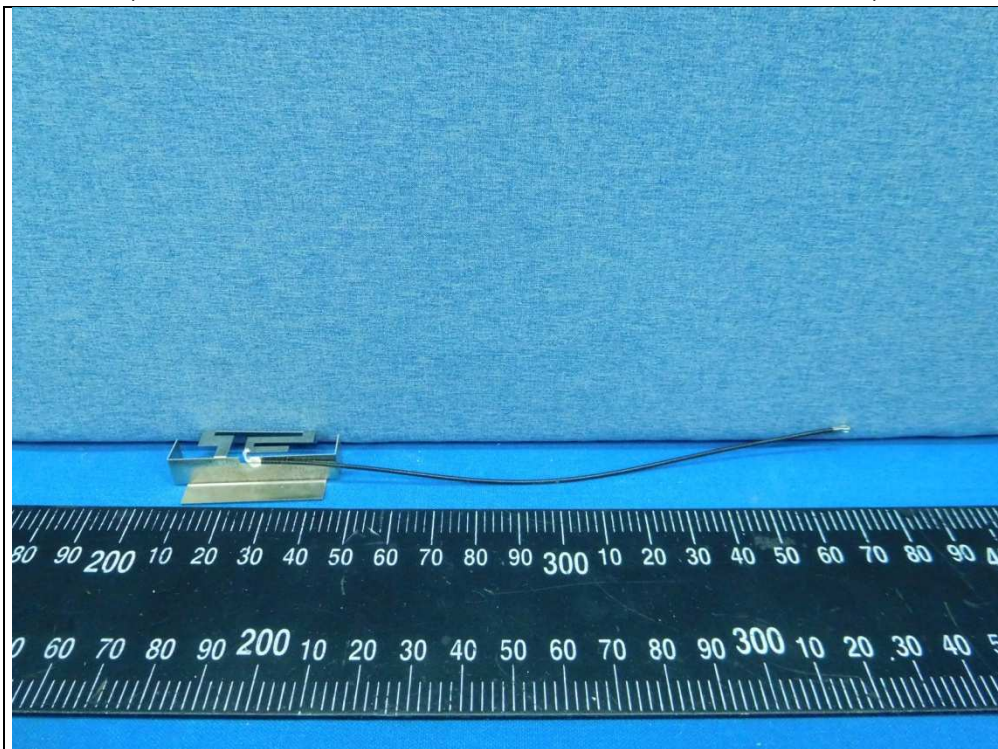
pex(MHF) Antenna (Brand: MAG.LAYERS Model: MSA-4008-25GC1-A2)
