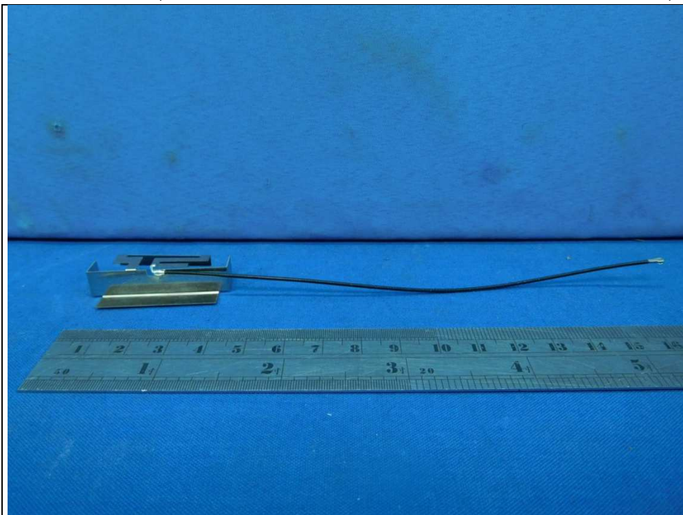
PIFA Antenna (Brand: MAG.LAYERS Model: MSA-4008-25GC1-A1)
