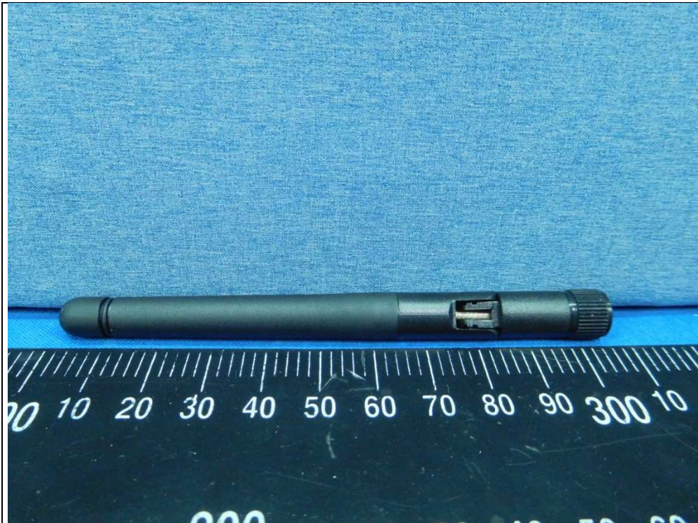
Dipole Antenna (Brand: Chang Hong Model: DA-2458-02-SMR)
