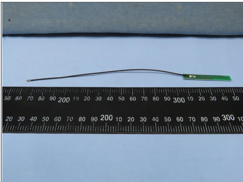
Antenna Set 16(Brand: Nissei Limited, Model: FML2.4W45A-160-MHF4L)
