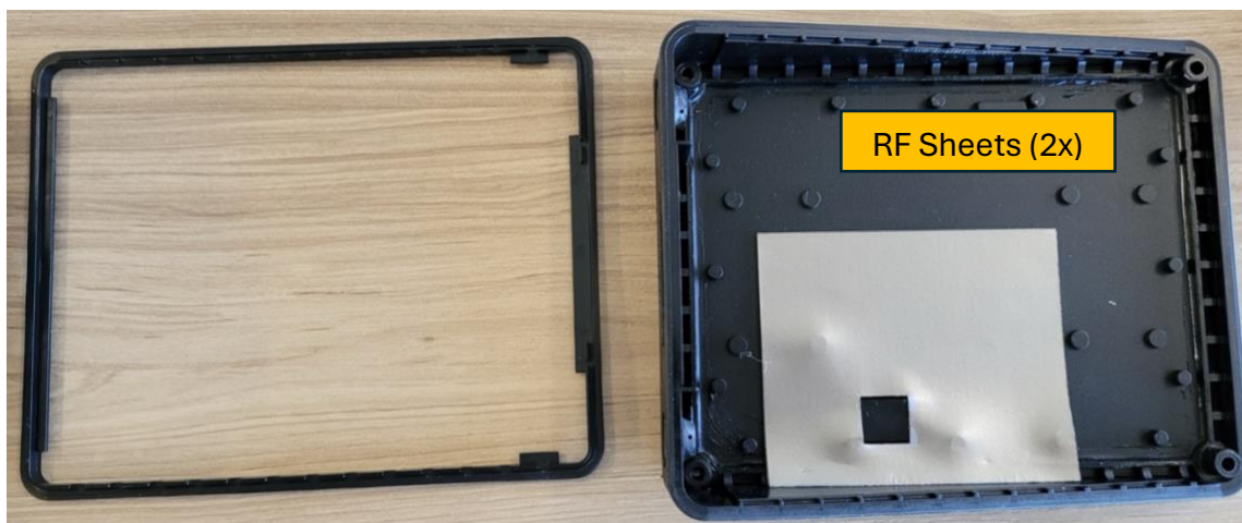
Opened case and gasket, Bottom of case
