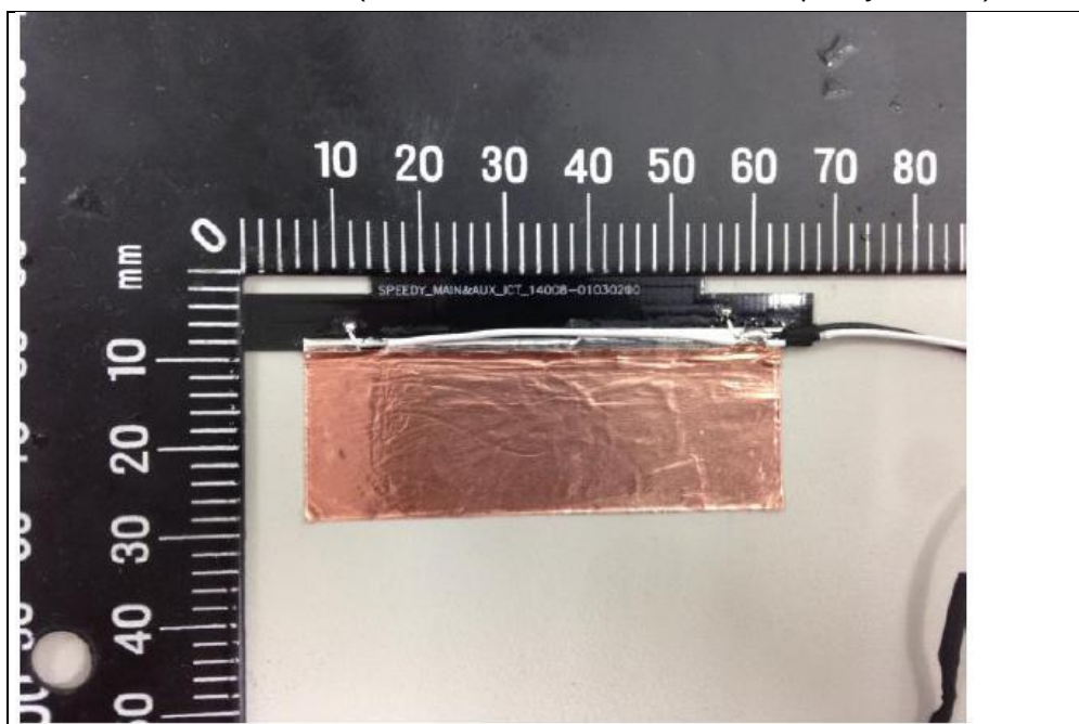
Antenna Set No.: 2 (Brand: LUXSHARE ICT; Model: Speedy <Main>)
