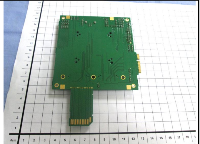
Rear Face
