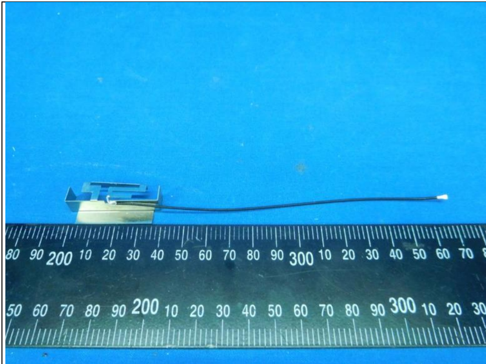
Antenna 1 (Model: MSA-4008-25GC1-A2)
