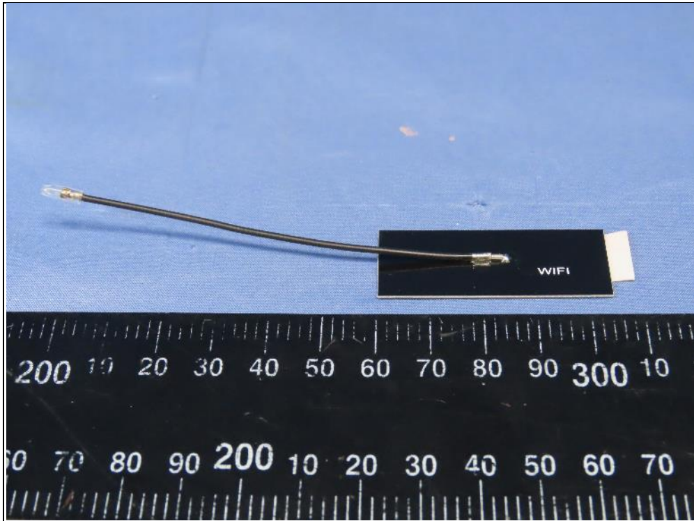
Antenna 3 (Model: EA-2INP501-0010)
