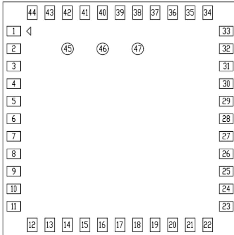
AW-CM358 Top View Pin Map
