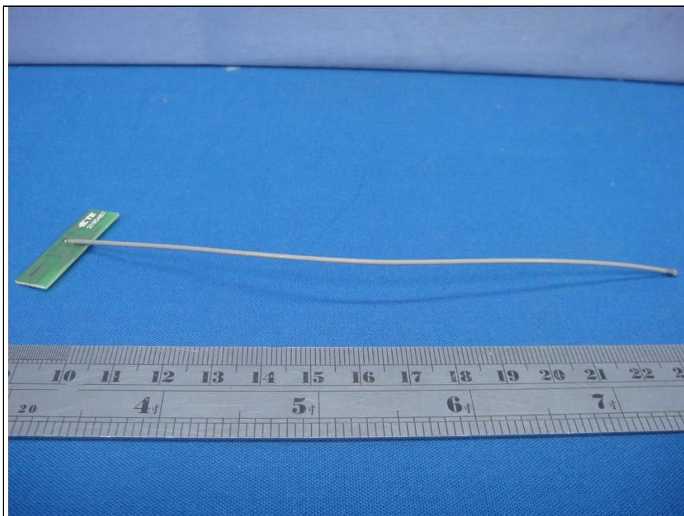
Set 3 Antenna (Model No.: 2195487_ Dipole / Brand: TE connectivity)
