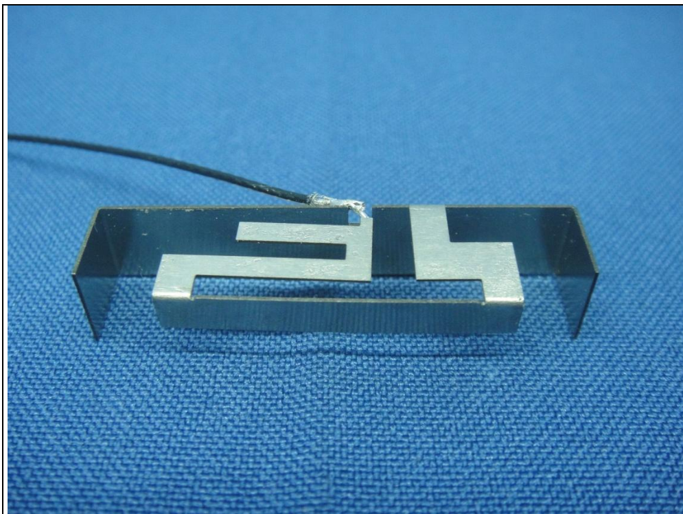
Set 1 (Model No.: MSA-4008-25GC1-A1 / Brand: MAG.LAYERS)
