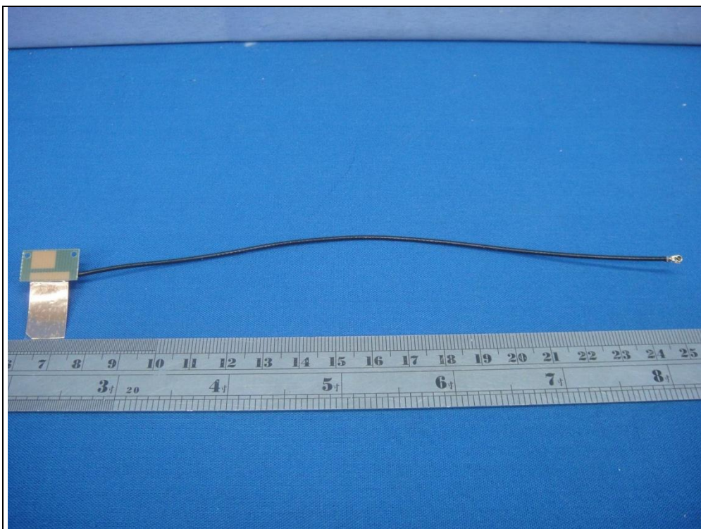
Set 4 Antenna (Model No.: 2195501-1_ Slot / Brand: TE connectivity)
