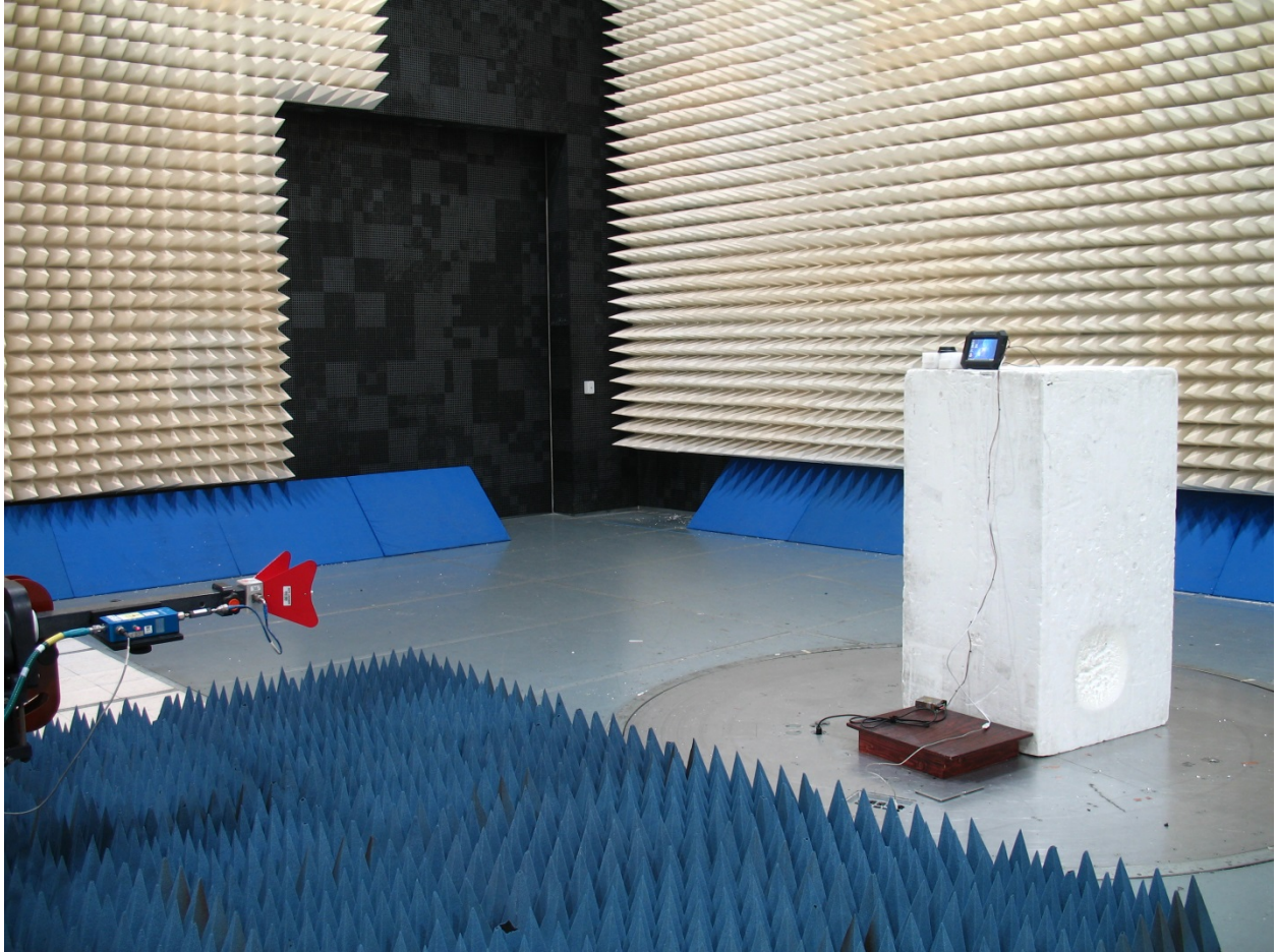
Setup – Spurious Emissions
