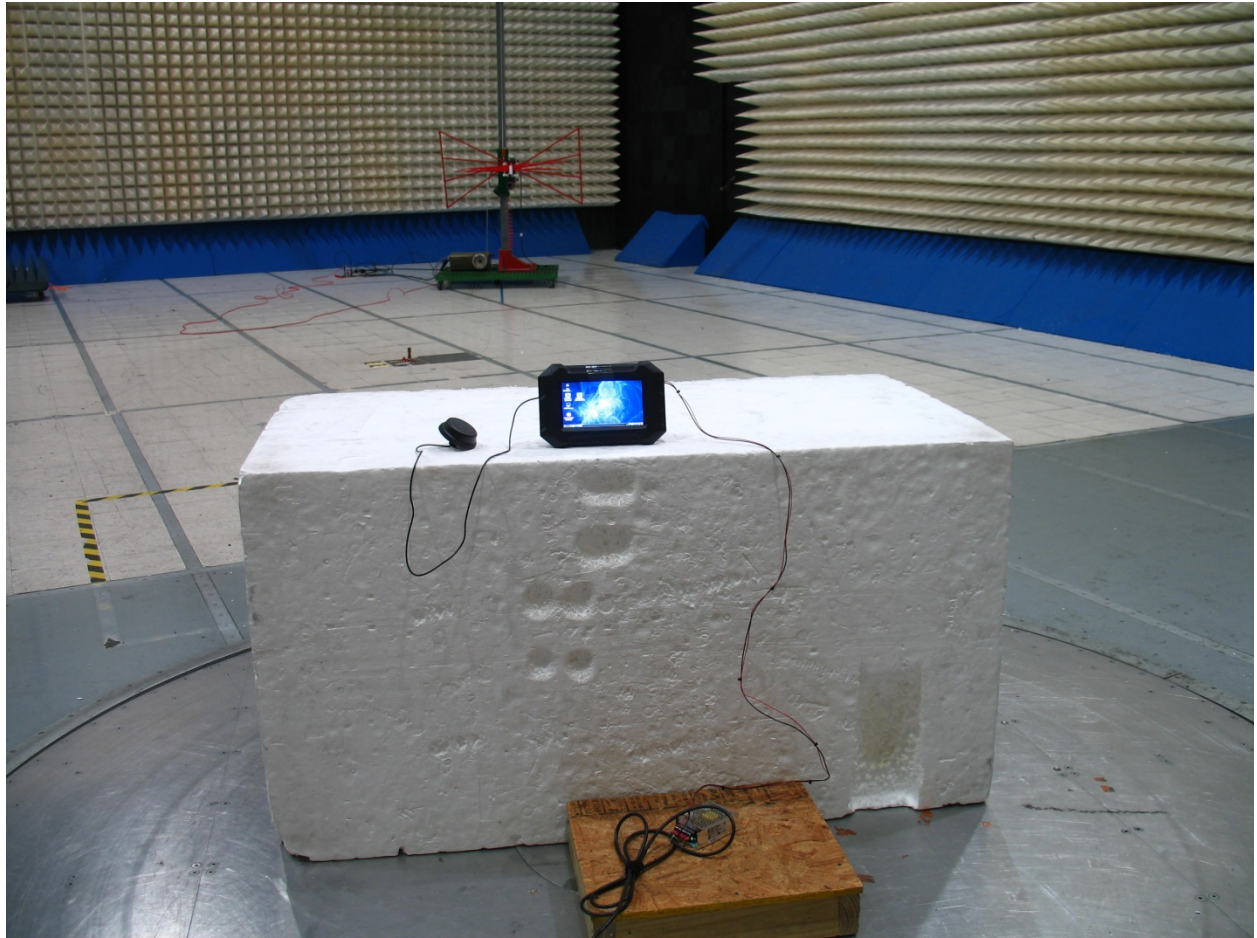
Setup – Radiated Emissions
